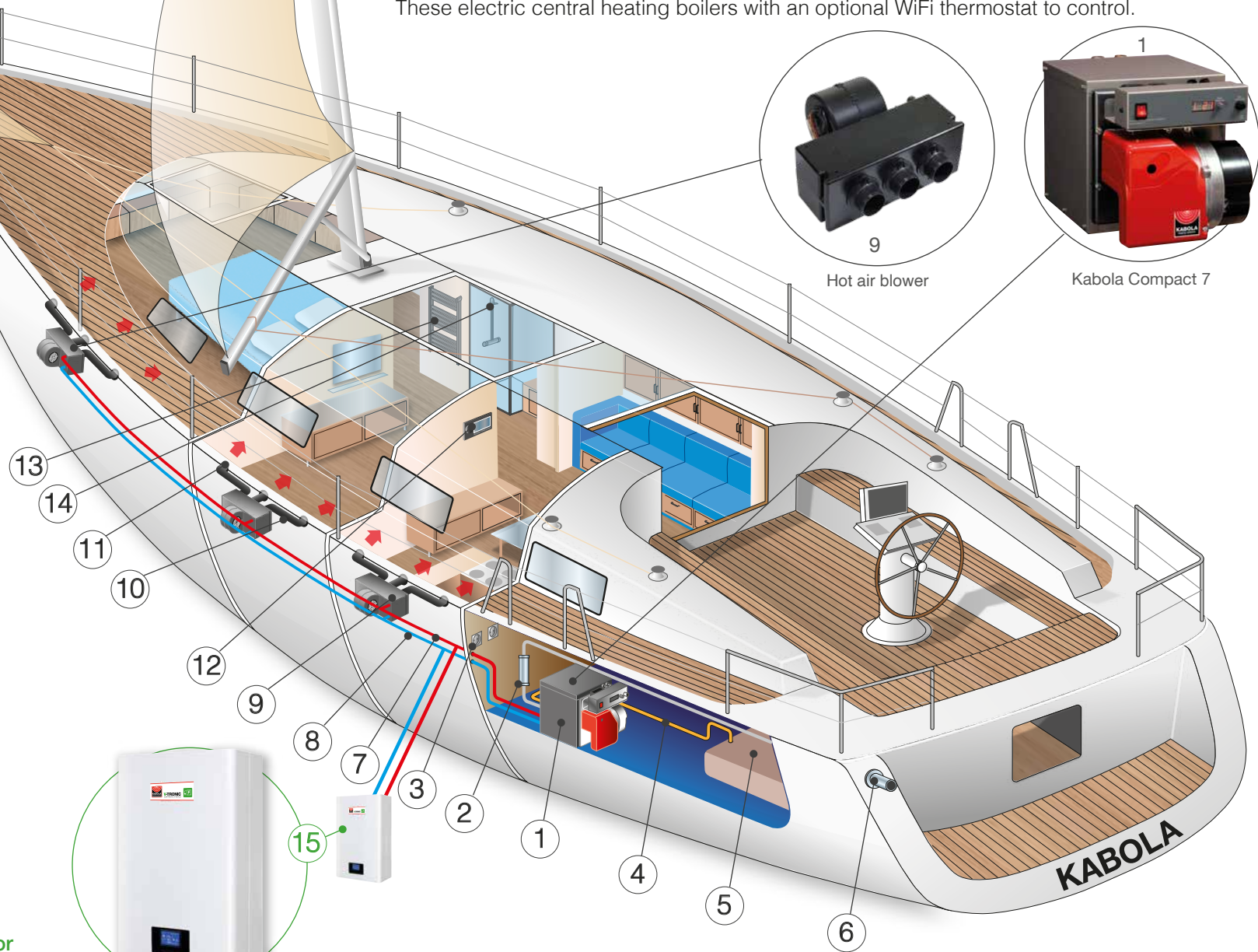
V-Tronic electric CH (combi)boiler
